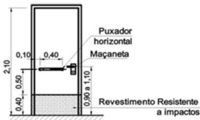
Vista frontal
